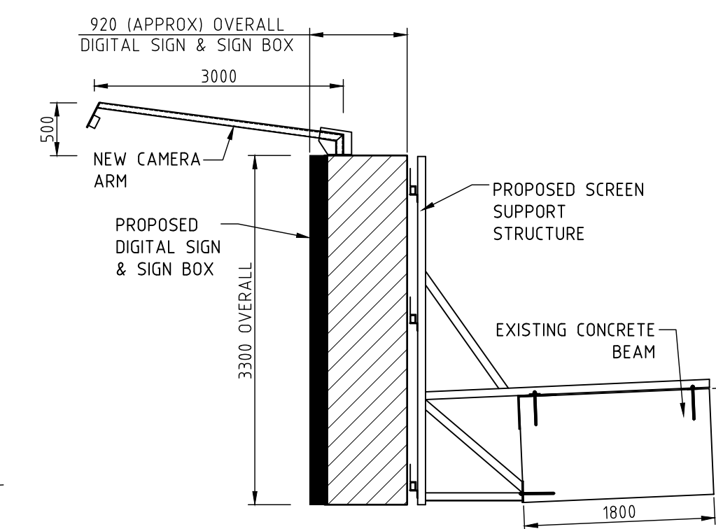
SECTION 2 SCALE 1:50
